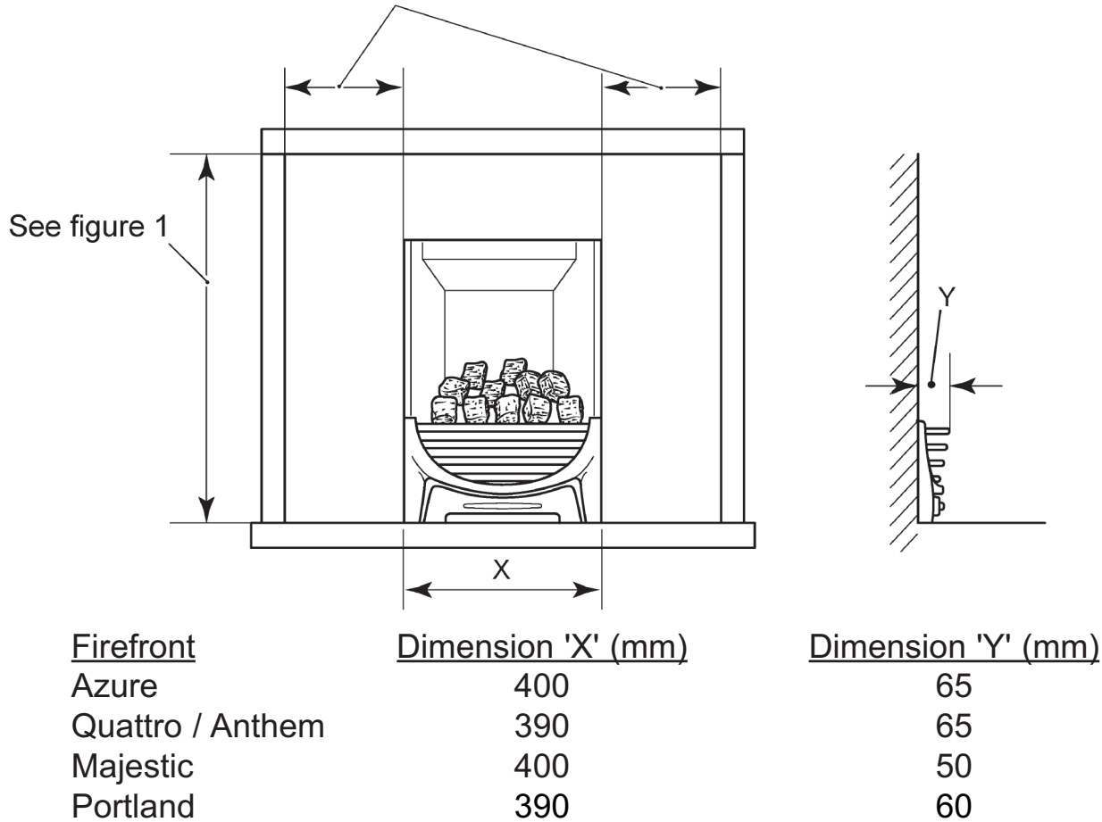
Figure 2. Appliance dimensions (Firefront may differ from that shown)
